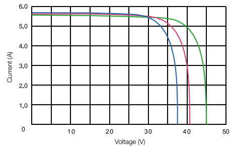
TP572M Pm(W)195
