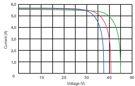
TP572M-B Pm(W)195
