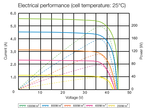
TP572M-B Pm(W)195
