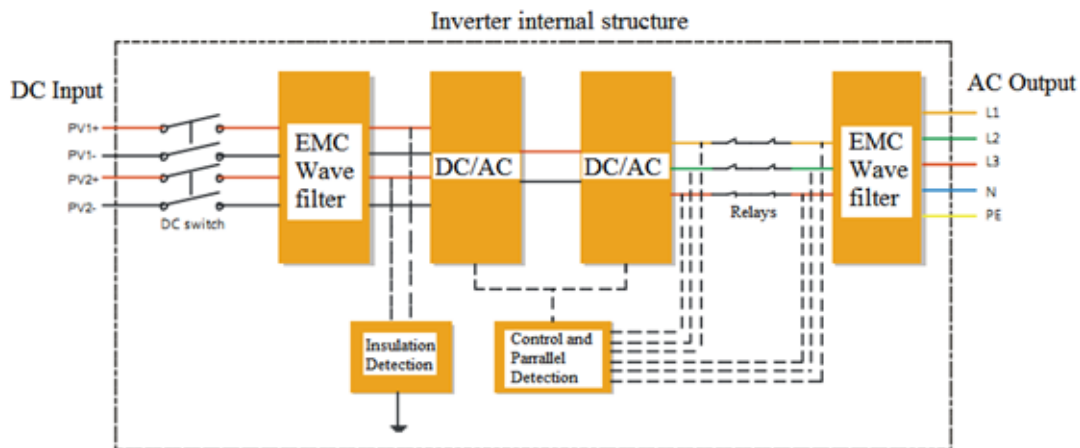
Figure 1. Inverter Internal structure
